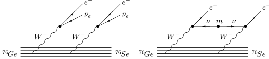
Fig. 10.2. Two neutrino and neutrinoless double beta decay
